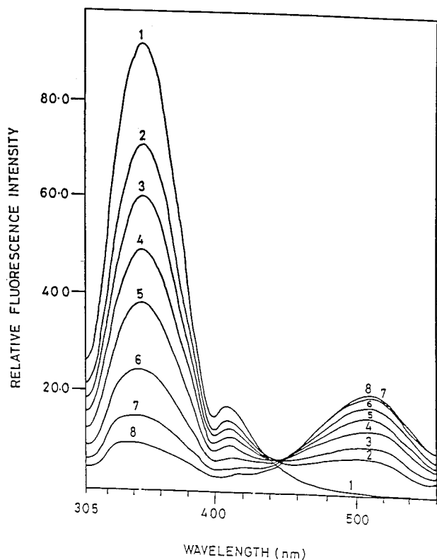
FIGURE 1: Fluorescence energy transfer from acid-unfolded cytochrome c to ANS at pH 2.0. Fluorescence emission spectra of samples with 7 \mu M cytochrome c in the presence of (1) 0, (2), 2.5, (3) 5, (4) 7.5, (5) 10, (6) 15, (7) 20, and (8) 25 ANS:protein (mol: mol) in 20 mM HCl scanned at 27 °C. The excitation wavelength was 290 nm. All measurements were carried out after the samples had been equilibrated for 3 h at 27 °C.
